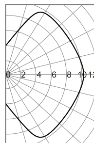
Figure 3: Detection characteristics of GBS detector.
